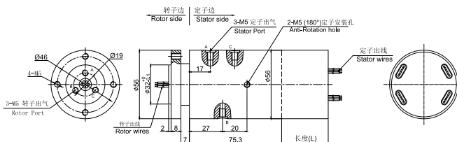
MAPH300-01+Electricity size
